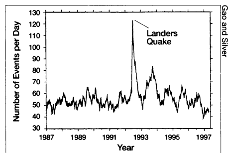
Western U.S. earthquakes have exhibited a yearly cycle since the Landers jolt.
