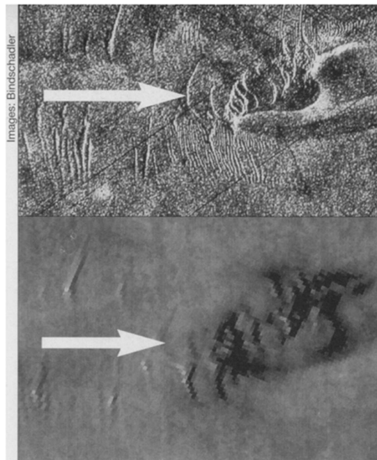
Satellite images from 1963 (top) and 1980 track the movement of a crevasse (arrows) in Ice Stream B.
