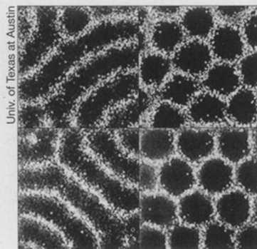
These images compare patterns resulting from computer-simulated vibrations of granular materials (top) with those from experiments using small lead spheres (bottom).
