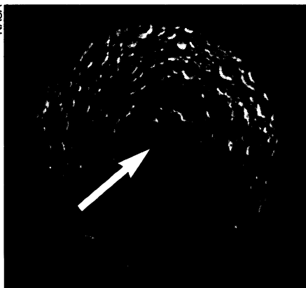
The moon's south pole, imaged by Clementine, shows a crater (arrow) that may contain ice.
