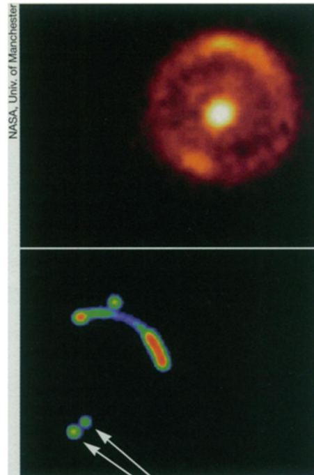
Top: Hubble picture shows an image of a distant galaxy distorted into a ring by a galaxy nearer Earth (center of ring). Bottom: MERLIN observation shows two radio sources (arrows) in the distant galaxy. The arc and the blob just above are lensed images of these sources.
