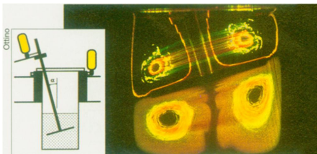
Fluorescent dyes illuminated by a sheet of laser light expose a vertical cross section of a liquid flow pattern in a mixing tank. Dark areas represent relatively quiescent regions of poor mixing, whereas stretched and folded dye streaks indicate chaotic regions of good mixing. Inset: A motor (yellow on left) rotates a tilted disk, which generates two rings of moving liquid, one above and one below the disk.
