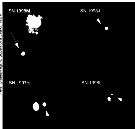
Four distant supernovas (arrows).
