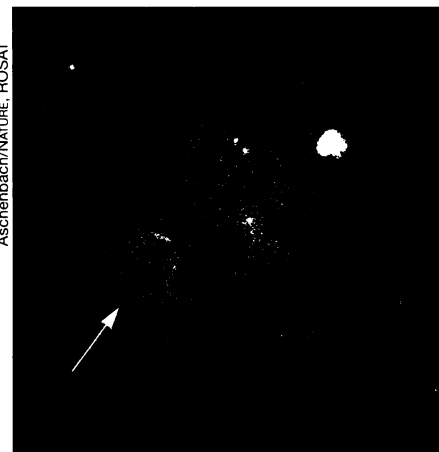
A young, nearby supernova remnant (arrow).
