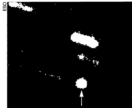
Image of 1996 TO66 (arrow) compiled from a total of 4 hours of exposure.
