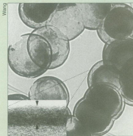
Carbon calabashes about 0.5 micrometer in diameter can be hollow or filled, as shown by this transmission electron micrograph. Graphite layers form the 8-nanometer-thick walls (arrows in inset).
