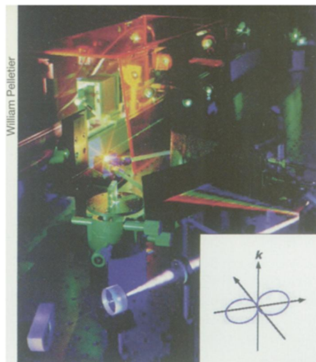
Accelerated by beams from this University of Michigan laser, electrons whiz through figure-eight patterns (inset) at right angles to the beam's direction of travel ( k ).
