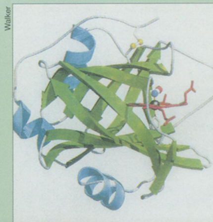
Components forming the three-dimensional complex nitrophorin 1. A heme molecule (red) sits at the opening of a barrel-shaped protein (green and blue ribbons). A molecule of nitric oxide (blue- and red-ball figure) binds to an iron atom (black) in the heme.
