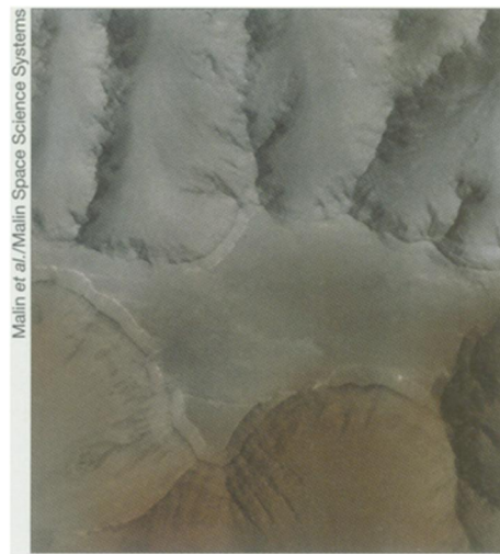
Layered material along the walls of the canyon Valles Marineris could be a sign of copious volcanic activity on early Mars.
