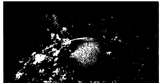
Reefs and carbon dioxide: Not a gas.
