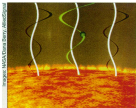
Surf's up: Observations suggest that the charged particles that make up the solar wind (red and green spirals) hitch a ride on magnetic waves in the sun's atmosphere, which drive the particles into space.
