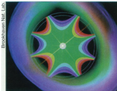
The magnetic field around the collider beam (white dot) must vary little. Green area around the beam is within proper range.
