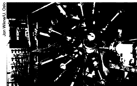
This instrument, called CACTUS, detects helium particles and gamma rays emerging from excited nuclei that undergo low-energy transitions.
