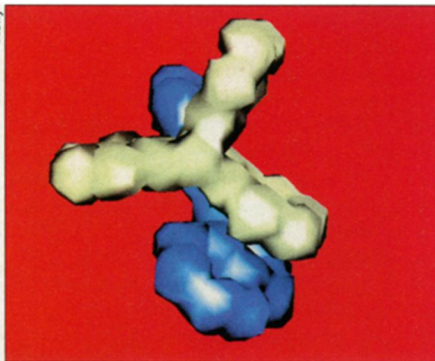
A one-way molecular motor consists of a three-bladed fan (white) attached to a ratcheting mechanism (blue).
