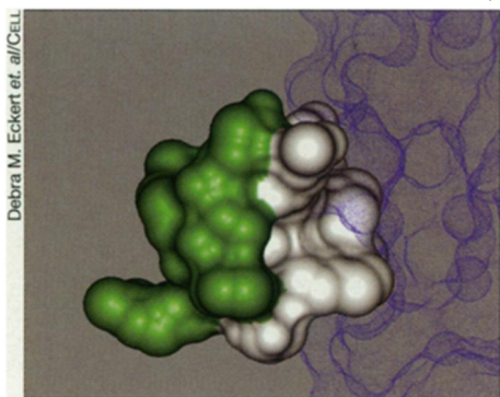
A possible AIDS drug (green and white) fills a pocket on an HIV protein (blue).
