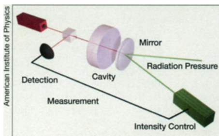
A laser (left) sends a light beam into an optical cavity, where it's reflected by a moving mirror and then deflected to a detector. That signal modulates the intensity of another laser beam (right), which exerts sufficient pressure to freeze the mirror's motion.
