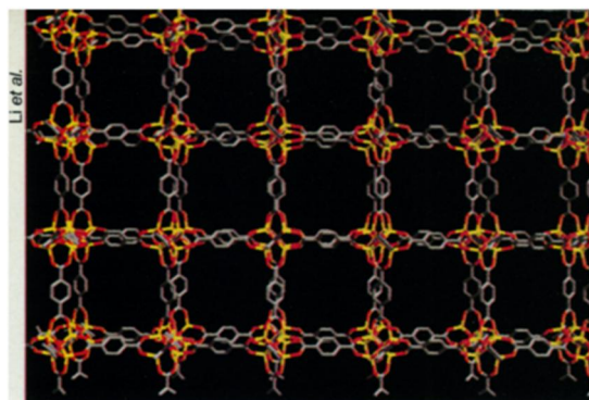
MOF-5 crystal architecture. Red is oxygen; gray, carbon; yellow, zinc. Clusters of 23 atoms form the nodes. Benzene rings are the struts. Cavities are about as wide as 8 water molecules. In this diagram, absence of electron clouds exaggerates the amount of empty space.
