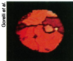
An unusual, high-pressure form of solid oxygen has a distinctive red color.
