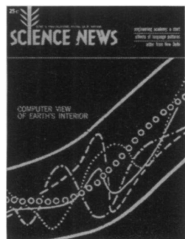
Some five million models of earth's structure, generated in a computer by a Monte Carlo method devised by Dr. Frank Press, turned up six that fit what is known about earth. Four of these show surprisingly high density variations in the mantle, as the white curves show. p. 551. (Photo: Dr. Frank Press).
