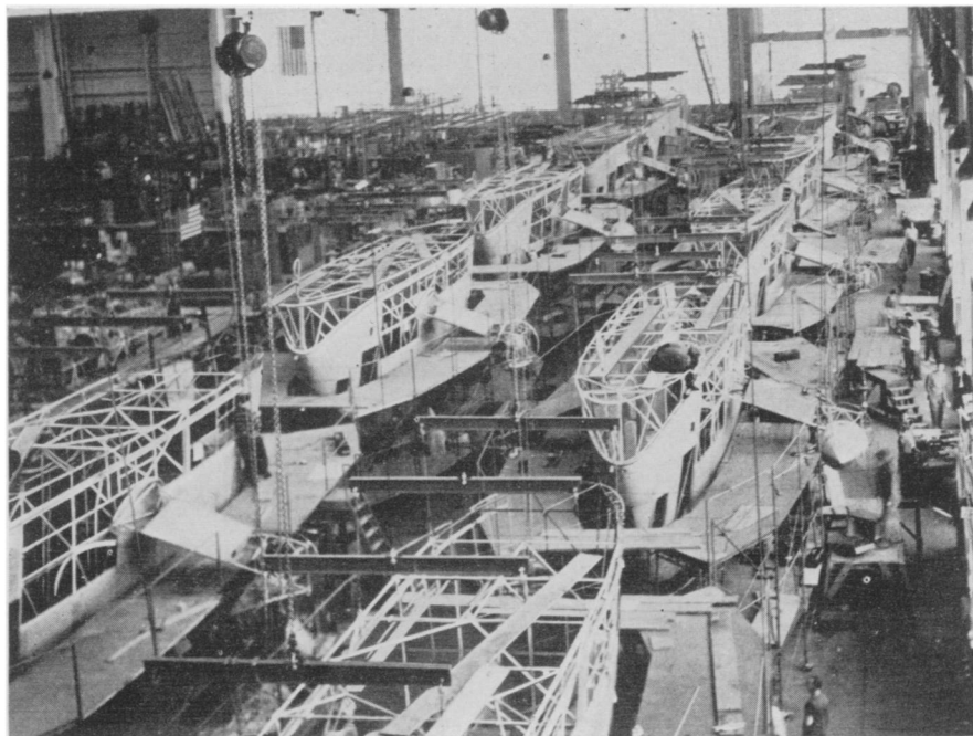
BLIMP CARS —This is just a portion of a long production line at the Good-year Aircraft Corporation plants in Akron where the streamlined control cars for U. S. Navy blimps are being assembled. Construction at the beginning of the line starts with the cars inverted. Half way through, they are turned over, as shown here, for attaching the motors to the outriggers and for other final touches.
