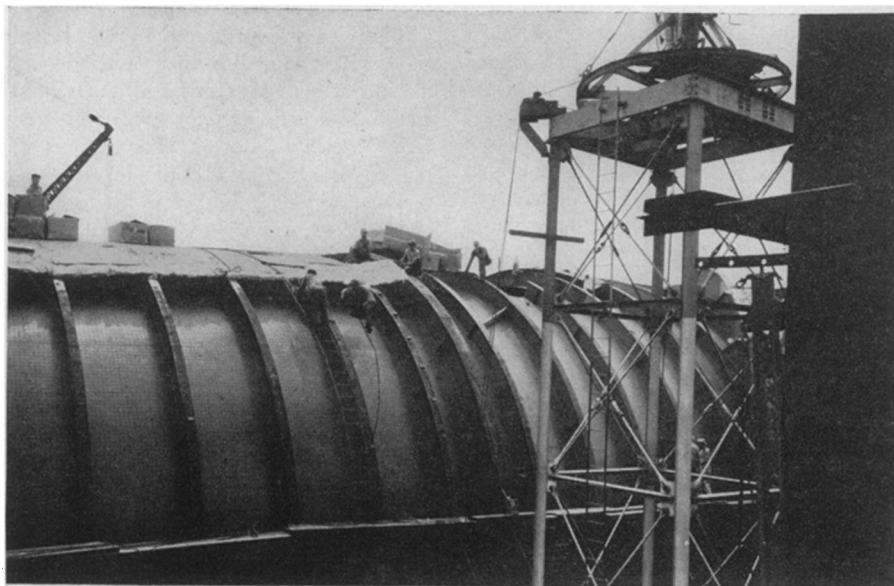
FIRST OF ITS KIND —This is the NACA's new and unique altitude wind tunnel under construction at the Cleveland Airport. The tunnel is insulated by fiber glass.
