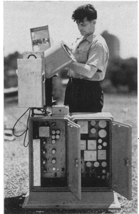
CHECKS CEILING — Airplane pilots can have continuous information about the height of the clouds by means of this instrument, the ceilometer, shown here with Laurence W. Foskett, of the U. S. Weather Bureau, one of the inventors.
