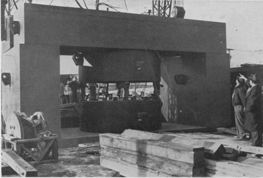
CYCLOTRON MAGNET —Giant steel blocks, forged by the United States Steel Corp., are assembled to form the magnet for the University of Rochester's cyclotron, second largest cyclotron in existence. Finished, the four forgings making the base and top weigh 157 tons each, the side columns 125 tons each, and the round pole pieces 90 tons each.
