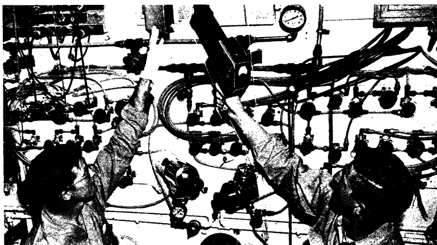
CHECKING RADIATION —Fission product materials emitting high levels of radiation are processed inside a thick walled concrete cell. This shows apparatus on the outside wall where all operations are performed by remote control. Radiation emitted through an opening is being checked with an instrument called a "cutie pie."
