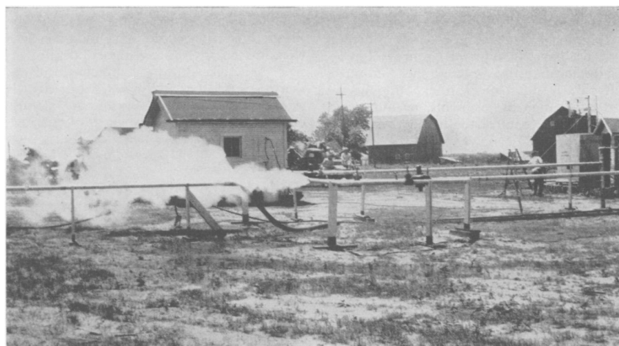
GASIFICATION TEST —Gas is escaping from the pipe sunk into the coal in the production of fuel gases from unmined coal by the use of electricity. This method eliminates the "cost of mining" factor.
