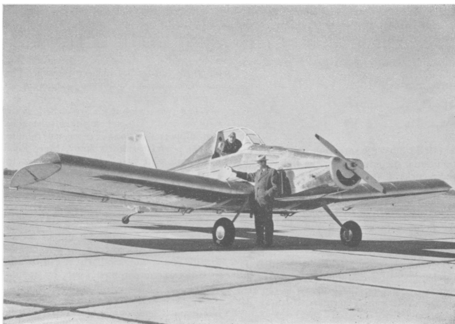
INSECTICIDE TANK —This little airplane is designed especially for dusting, spraying, seeding or fertilizing farm crops. Fred E. Weick is shown opening one of the spray tanks.
