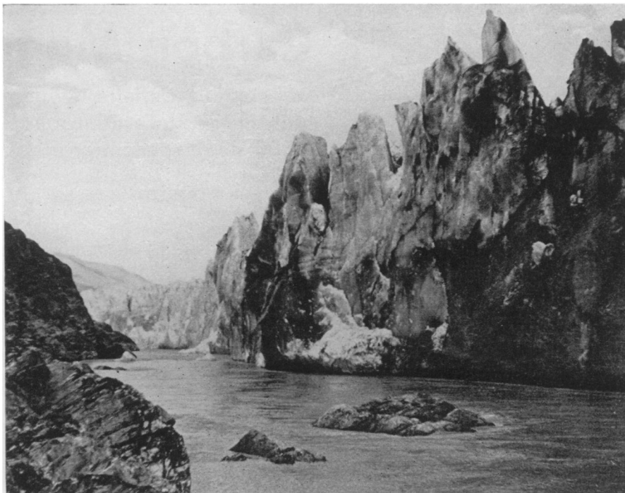
SELF-DUMPING LAKE —Lake George, in the mountains of southeastern Alaska, dumps itself about Aug. 1 of each year, dropping the water level by more than 100 feet. Details of the water flow through a gorge in the ice and into the sea were studied last summer by Prof. Kirk H. Stone of the University of Wisconsin.
