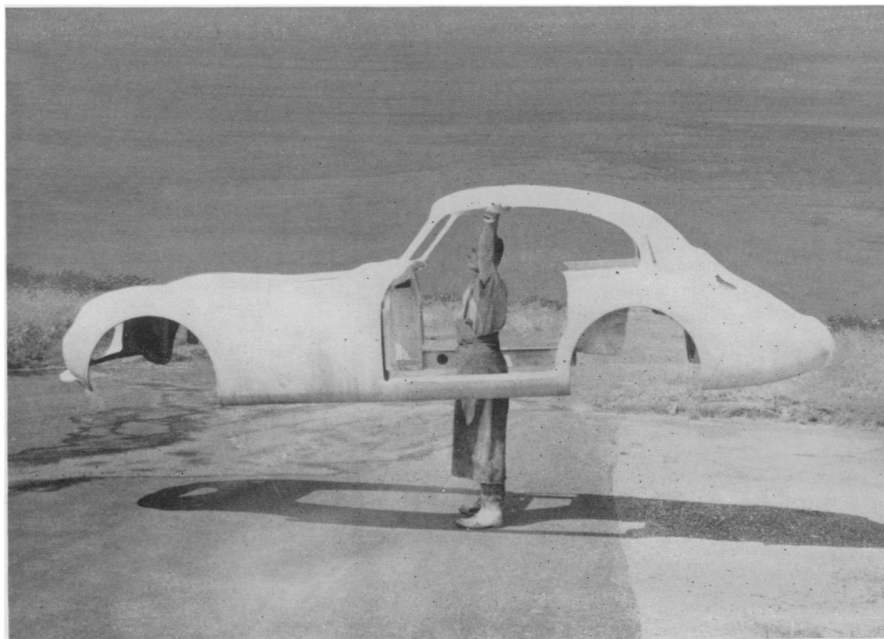
ALL-MAGNESIUM AUTO BODY —Weighing only 132 pounds, this auto body made entirely of magnesium was developed in England. It is mounted to the chassis at only six points.
