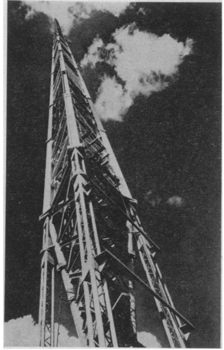
TV TOWER — The world's tallest television tower, now nearing completion, is shown here. The triangular 1,572-foot transmitter for station KWTW, Oklahoma City, is 12-foot on a side up to the 1,420-foot level. From there it tapers to the base of the antenna.
