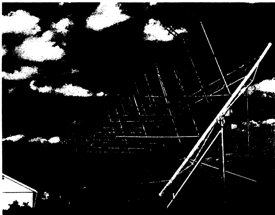
MESSAGES FROM SPACE —Ohio University's radio telescope was one of the four instruments to fix the center of our galaxy. The giant antenna picks up radio waves from space. With it astronomers can "see" some parts of the universe where light telescopes cannot penetrate.
