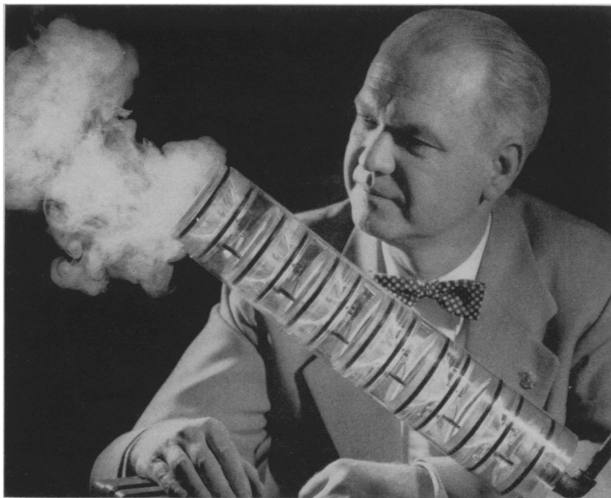
MEASURING PARTICLE SIZE —To measure the size distribution of particles dispersed in air, the cascade impactor shown here was developed by scientists at Battelle Memorial Institute, Columbus, Ohio, for the Army Chemical Corps. Increasing speed and inertia are imparted to particles as aerosols are drawn through a series of funnels with successively smaller openings. When the inertia of the particles overcomes air drag, they impact on the various slides for later detection.
