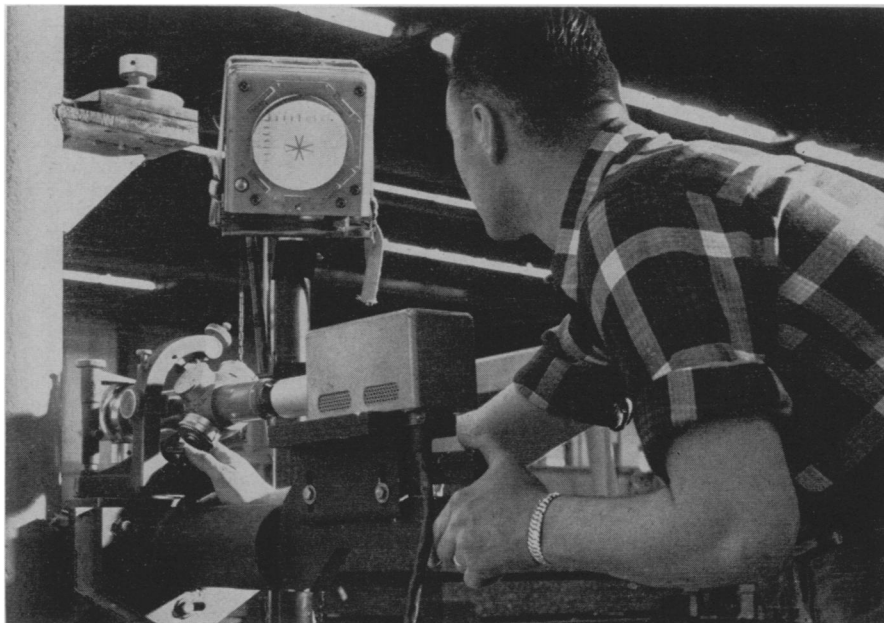
TV OPTICAL TOOLING —A closed circuit television system that can cut costs and speed production of supersonic fighter-bombers has been developed by Republic Aviation Corporation. Previously a two-man operation in an optical tooling process, now the TV camera automatically "looks" through the telescope while the operator positions jig contour plates by lining up cross-hair patterns as they appear on the TV screen.
