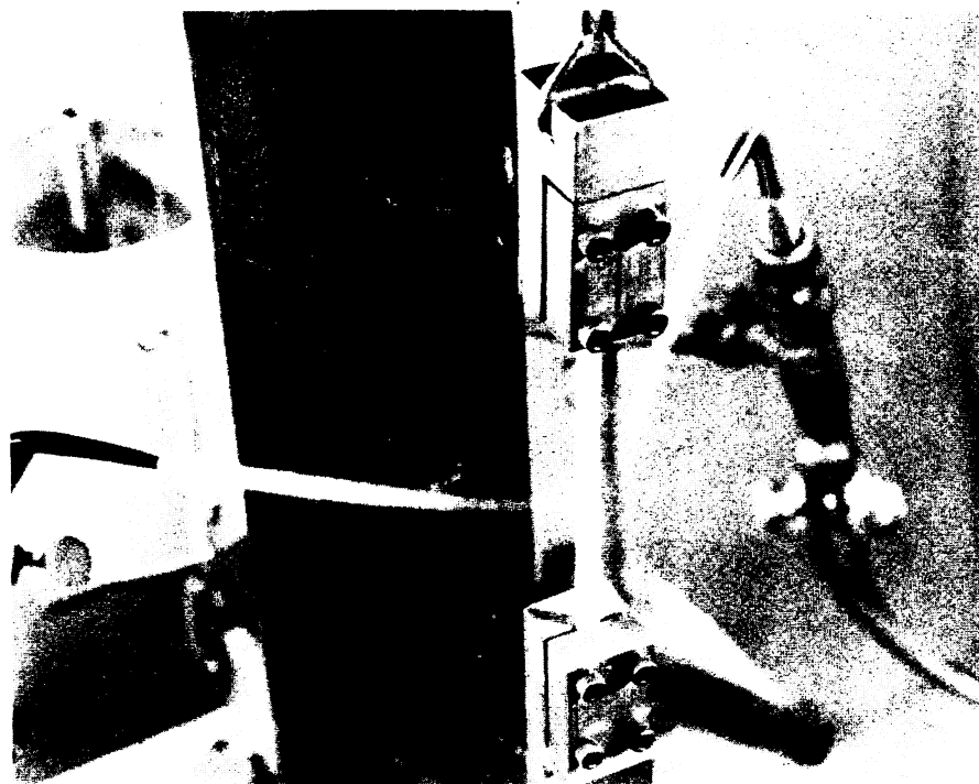
PYROCERAM —The rod of Pyrocera shown in the photograph can withstand the heat of two acetylene torches, with weights pulling at each end, and maintain its strength indefinitely. Flexural strengths as high as 80,000 pounds per square inch have been measured on some varieties of Pyrocera.
