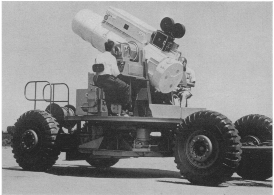
OPTICAL TRACKING SYSTEM —The telescopic photographic recorder, or TPR, shown in the photograph is the nation's first completely mobile, high-performance optical tracking system capable of photographing the flight of bombs, aircraft and missiles. The 70 mm motion picture camera is in position mounted on the telescope. It was developed and built by the Perkin-Elmer Corporation, Norwalk, Conn.
