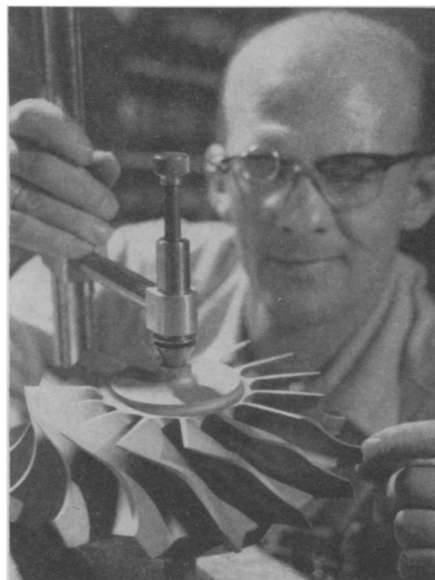
TURBINE WHEEL —This radial inflow wheel is made from Udimet 500, a superalloy, composed of heat treatable nickel-base alloy containing cobalt, molybdenum, chromium, titanium and aluminum. It is being tested at Boeing in Seattle.
