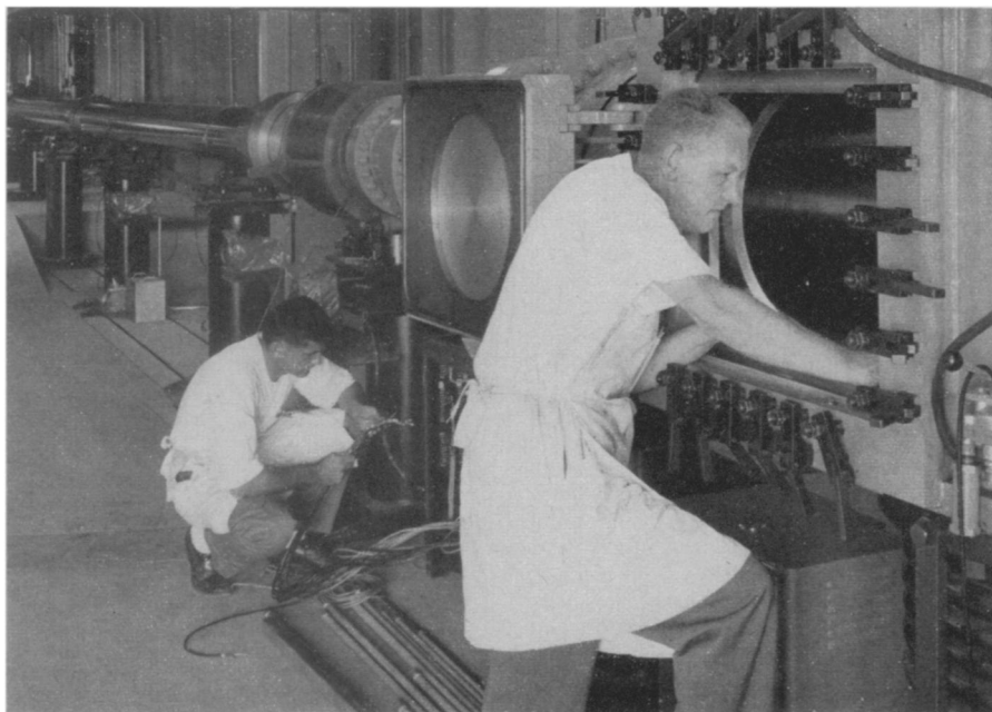
SHOCK TUNNEL —Used for testing aircraft and missile models at air speeds ranging from six to 16 times the speed of sound, the tunnel is almost 110 feet long. Technician (right) is working on the test section where a model is mounted during testing in the tunnel, developed by Cornell Aeronautical Laboratory, Inc., Buffalo, N. Y.
