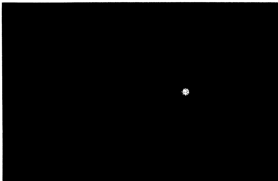
COMET IN FLIGHT —The Comet Burnham, taken by Dr. Elizabeth Roemer with the 40 inch reflector at the U. S. Naval Observatory at Flagstaff, Ariz. The comet's tail was one-fourth of a degree long when this picture was taken.
