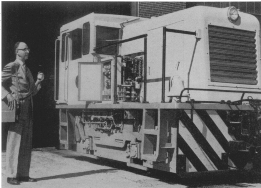
RADIO-CONTROLLED LOCOMOTIVE —All the functions of a normal diesel-electric locomotive will be controlled by a black box in the cab of the engine. Holding a transmitter for sending signals to the black box is J. W. Brauns of General Electric's Locomotive and Car Equipment Department in Erie, Pa.
