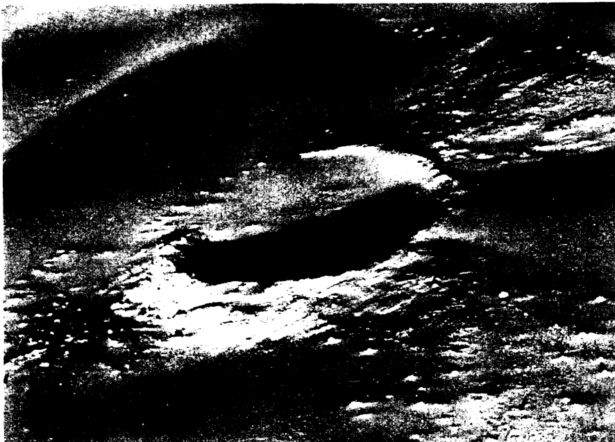
SITE OF COESITE —The fourth location in the world known to contain the rare mineral coesite is meteor crater Wabar (Al Hadida) in Saudi Arabia. Other locations are Meteor Crater, Arizona, Ries Crater, Germany, and an atomic bomb site at Yucca Flats, Nev.
