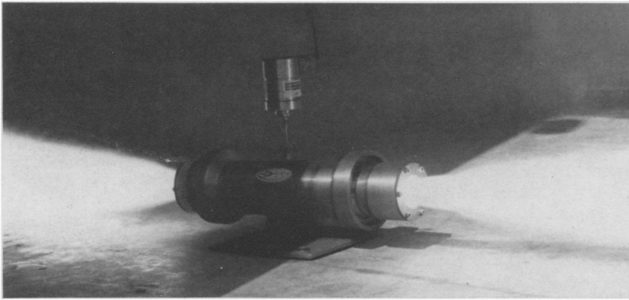
TWO HEADS ARE BETTER —A two-headed midget rocket motor that fires simultaneously from both ends has been developed to test new rocket nozzle designs and materials by the United Technology Corporation's Development Laboratory in Sunnyvale, Calif. The rocket motor has a single combustion chamber for its two nozzles. It is designated a "Janus" test motor, after the ancient double-headed Roman god of gates and doors.
