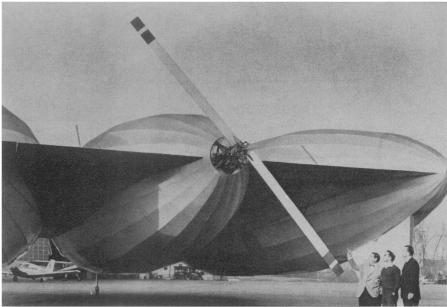
RIGID AIRSHIP —The multiple-bulbed Aereon , an experimental lighter-than-air craft, is powered by a helicopter-type rotor mounted at the stern of the center bulb. The dirigible incorporates new aerodynamic concepts, structural innovations and modern-day materials. Looking on are (left to right) Carl A. Beck, John R. Fitzpatrick and Monroe Drew Jr. of Aereon Corporation, King of Prussia, Pa.
