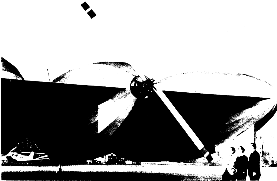
RIGID AIRSHIP —The multiple-bulbed Aereon , an experimental lighter-than-air craft, is powered by a helicopter-type rotor mounted at the stern of the center bull. The dirigible incorporates new aerodynamic concepts, structural innovations and modern-day materials. Looking on are (left to right) Carl A. Beck, John R. Fitzpatrick and Monroe Drew Jr. of Aereon Corporation, King of Prussia, Pa.
