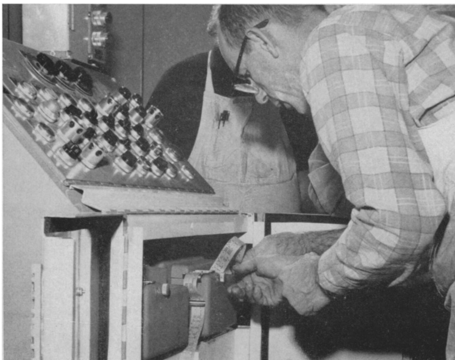
COMPUTER-CONTROLLED MACHINE —The photograph shows Lockheed Missiles & Space Company machinist E. A. Leb inserting a punched tape into the programmer that directs automatic milling of parts for the Navy's Polaris missile.
