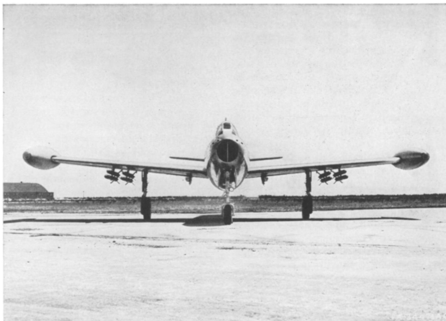
F-84 THUNDERJET —Eight, five-inch aerial rockets and six .50 calibre machine guns with 1,800 rounds of ammunition give this 600-mile-an-hour plane increased offensive power. After rockets are fired, the launching devices automatically retract to provide a streamlined wing surface.
