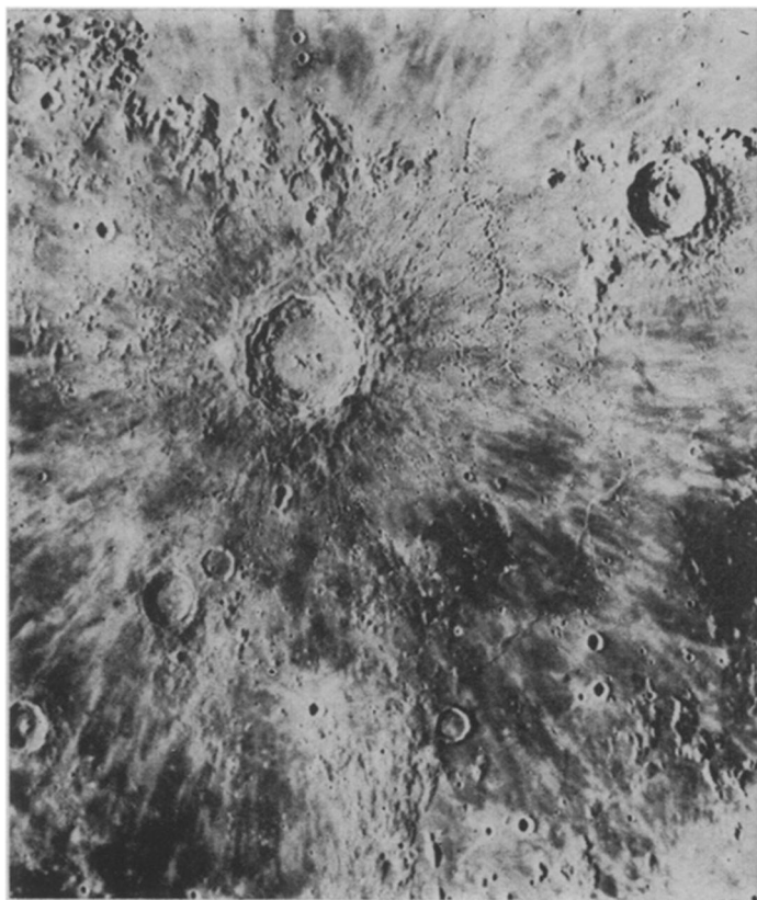
Lick Observatory
