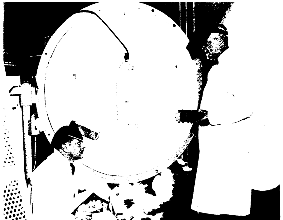
MEASURING MORE LIGHT —Scientists measure 150% more light in a new mercury lamp, developed by Westinghouse Electric Corporation, Bloomfield, N. J. The new lamp produces 78 lumens per watt compared to 54 of other mercury vapor lamps and 17 for incandescent lamps, such as ordinary light bulbs. The improvement was made possible when the rare element thallium was added to the mercury.
